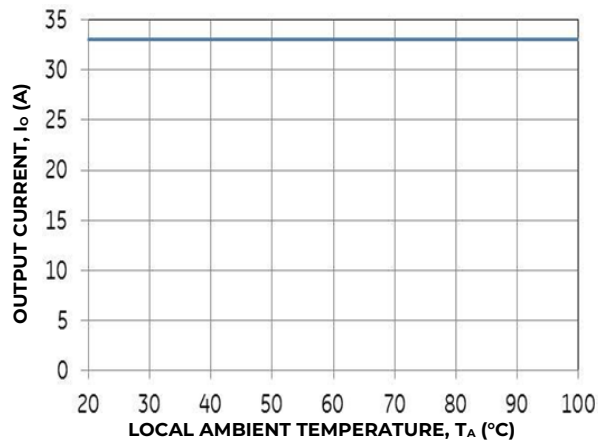
Figure 24. Output Current Derating for the Base Plate QBVW033A0B-H at 48V in in a Cold wall application; Local Internal Air Temperature near module=80°C; VOUT setting anywhere from 6.0V to 12.0V
