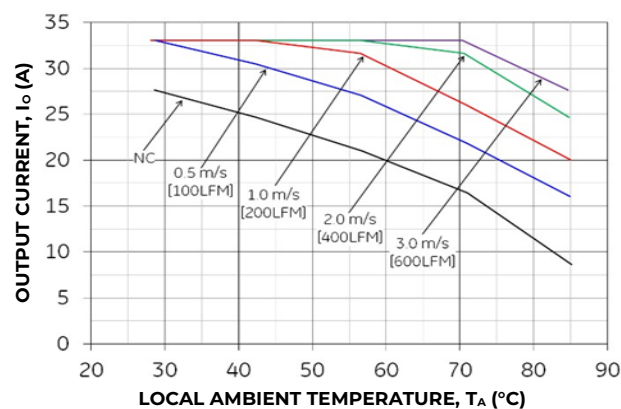
Figure 21. Output Current Derating for the Base plate QBVW033A0B-H at 48V in with 0.25" heatsink and Transverse airflow from V_{in}(-) to V_{in}(+)
