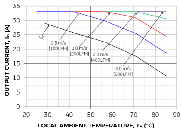
Figure 22. Output Current Derating for the Base plate QBVW033A0B-H at 48V in with 0.5" heatsink and Transverse airflow from V_{in}(-) to V_{in}(+)
