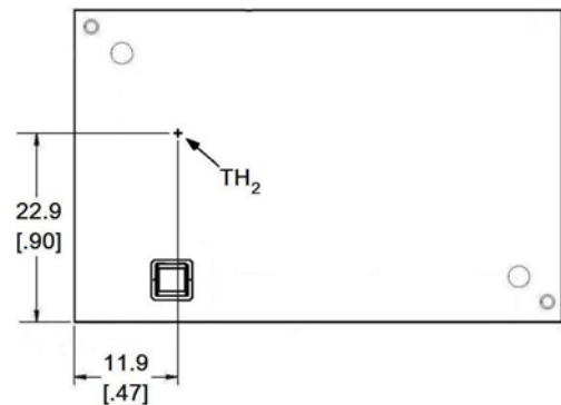
Figure 18. Location of the thermal reference temperature TH2 for baseplate modules
