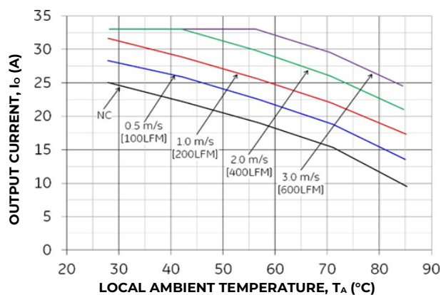
Figure 19. Output Current Derating for the Open Fram QBVW033A0B at 48V in with Transverse airflow from V_{in}(-) to V_{in}(+)
