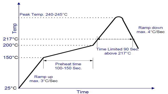
Figure 24. Recommended linear reflow profile using Sn/Ag/Cu solder.
