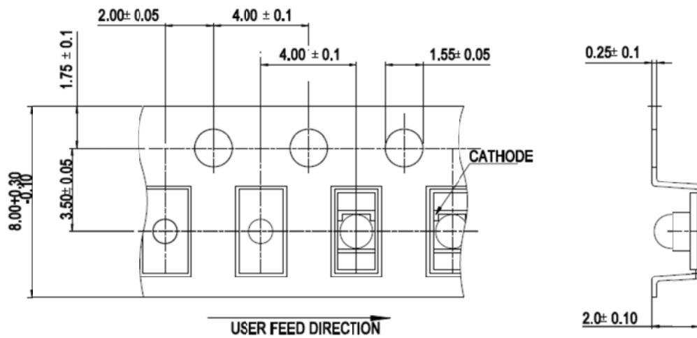
Figure 8: Carrier Tape Dimensions
