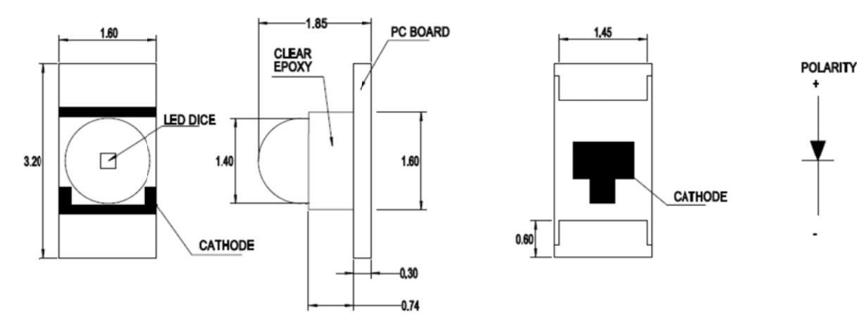
Figure 1: Package Dimensions
