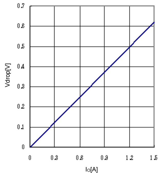
Fig.22 Minimum dropout Voltage 2 ( V_{cc}=4.5 V, T_a=25^{\circ}\text{C} )
