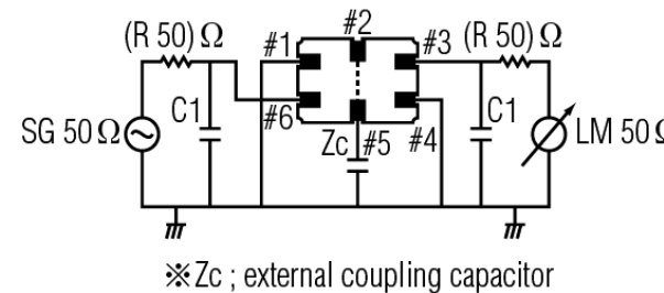
Figure 2) Test Circuit
