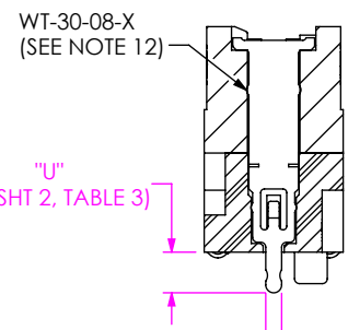
SECTION "M"-"M" SCALE 3:1
