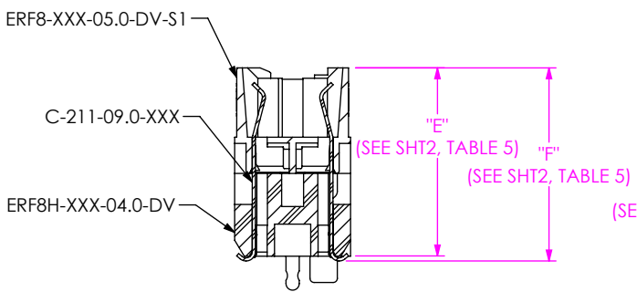
SECTION "N"-"N" SCALE 3:1
