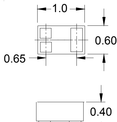
3 Pin SLP package (Bottom Side View) Nominal Dimensions in mm
