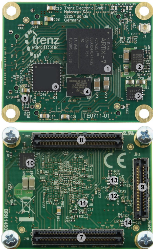
Figure 2: TE0711-01 PCB.
