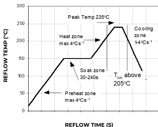
Figure 22. Reflow Profile for Tin/Lead (Sn/Pb) process.
