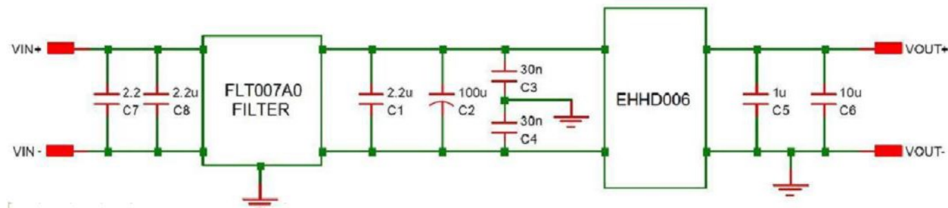
Figure 25. EMC Considerations
