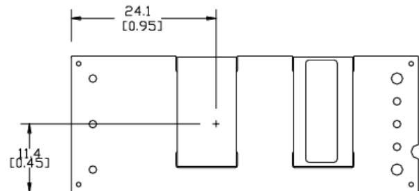
Figure 21. Pick and Place Location.
