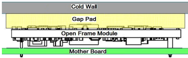
Figure 22. Cold Wall Mounting
