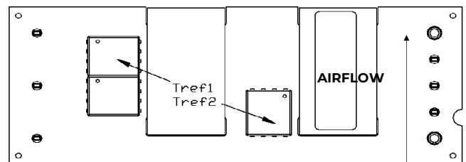
Figure 13. T_{\text{ref}} Temperature Measurement Locations for Open Frame Module.
