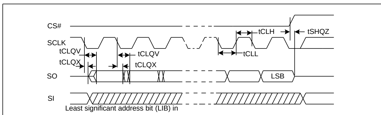
Figure 22. Output Timing
