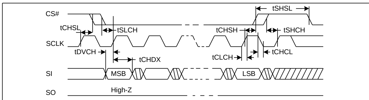
Figure 21. Serial Input Timing
