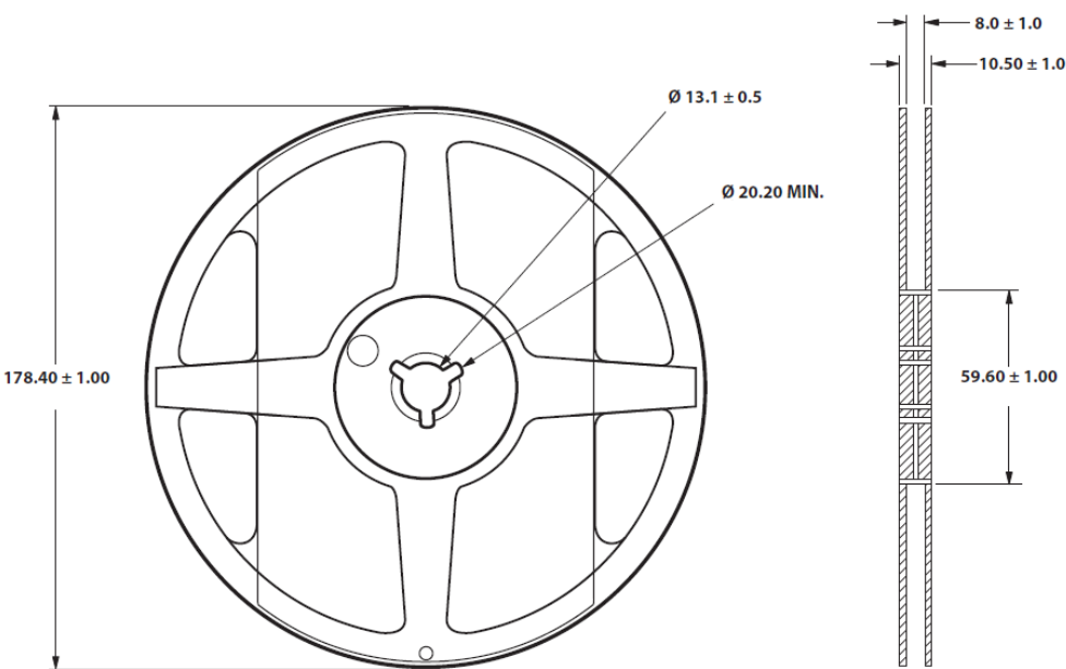
Figure 8: Reel Dimensions
