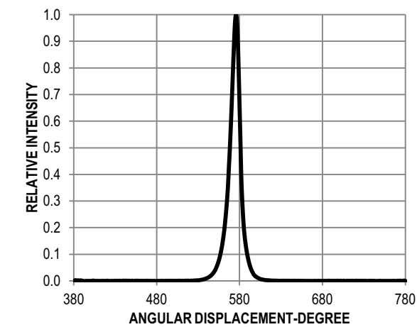
Figure 2: Relative Intensity vs. Wavelength
