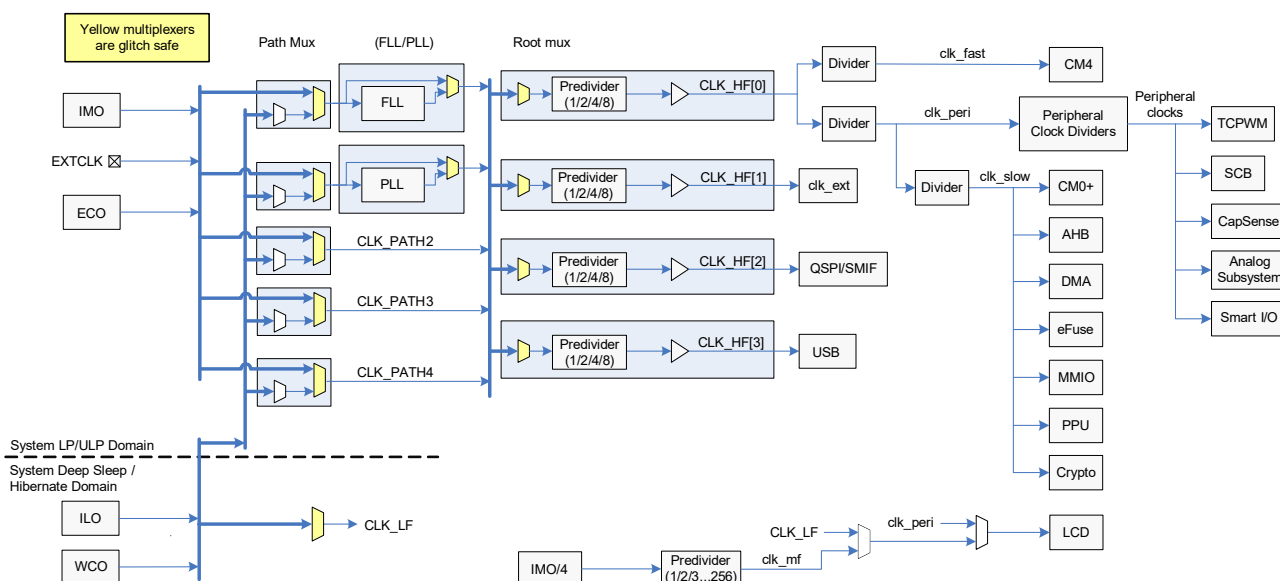
Figure 3. Clocking Diagram
