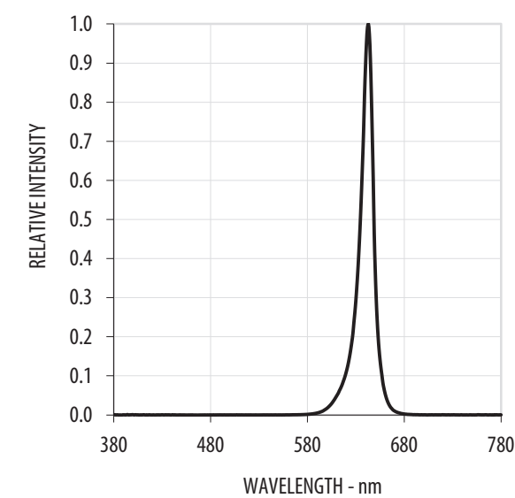
Figure 2: Spectrum
