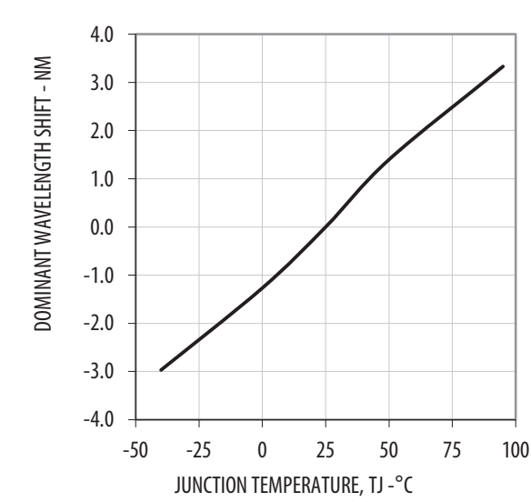
Figure 9: Wavelength Shift vs. Temperature
