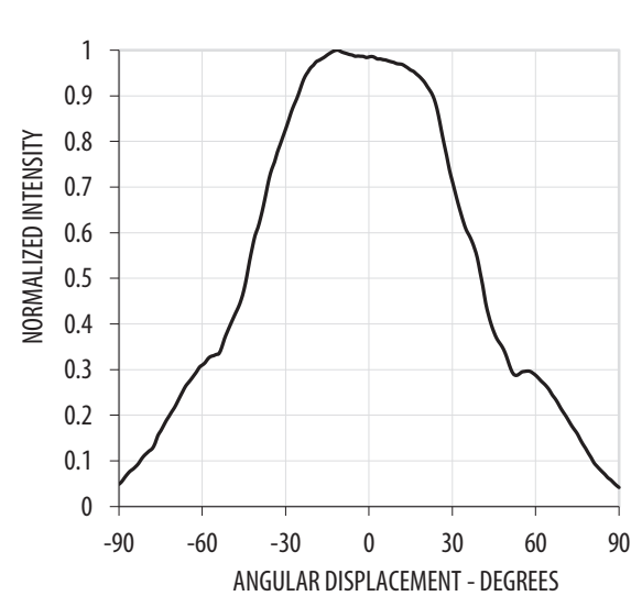
Figure 5: Radiation Pattern
