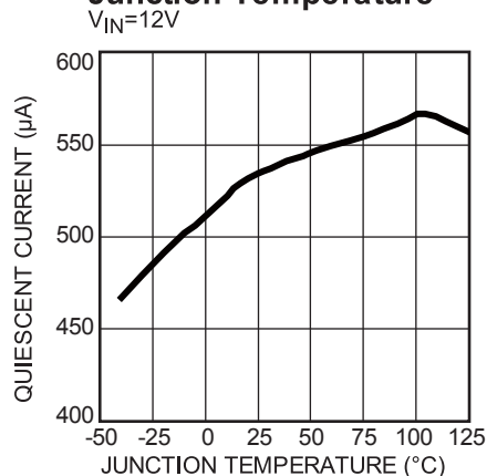
Quiescent Current vs. Junction Temperature V_{IN}=12V
