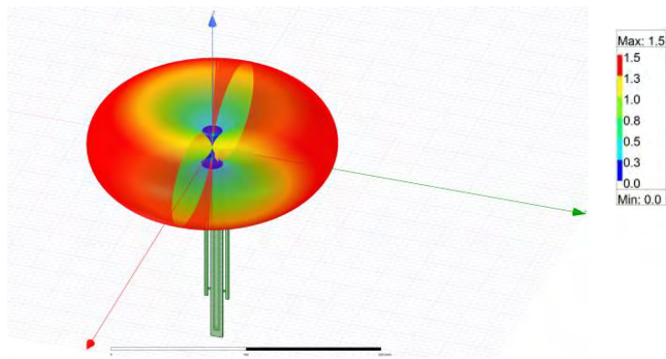
Radiation Pattern
