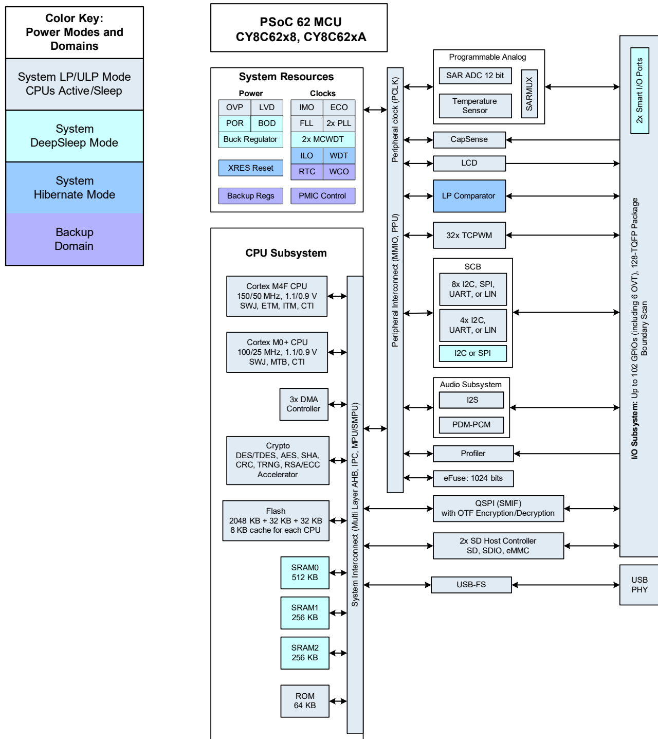
Figure 2. Block Diagram
