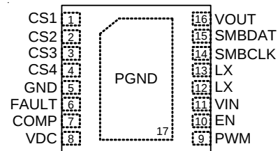
WDFN-16L 5x5
