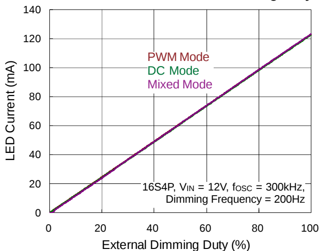
LED Current vs. External Dimming Duty
