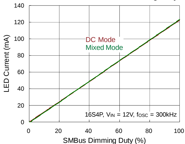
LED Current vs. SMBus Dimming Duty
