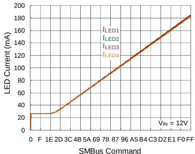
LED Current vs. SMBus Command
