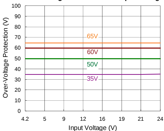
Over-Voltage Protection vs. Input Voltage
