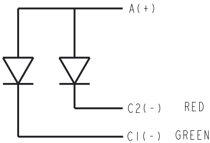
LED SCHEMATIC
