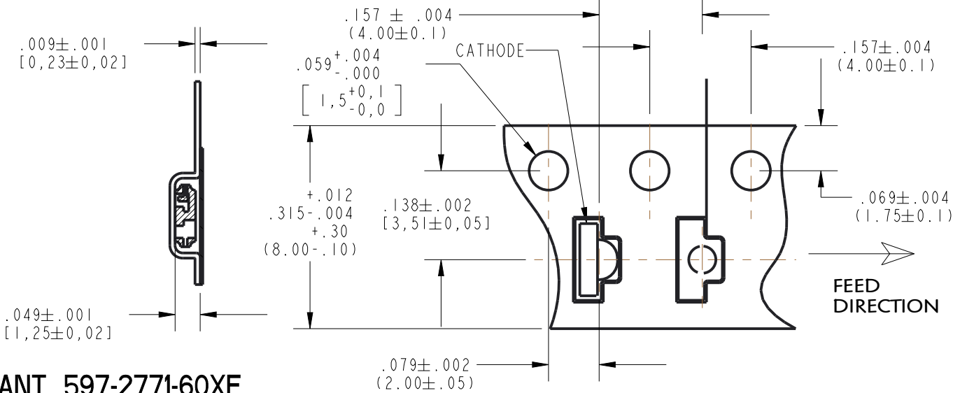
PACKAGE DIMENSIONS OF TAPE AND REEL (NO SCALE)
