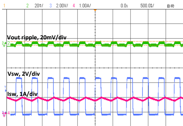
Output Ripple and SW at 1A load V_{\text{in}}=5\text{V} / V_{\text{out}}=1.8\text{V}
