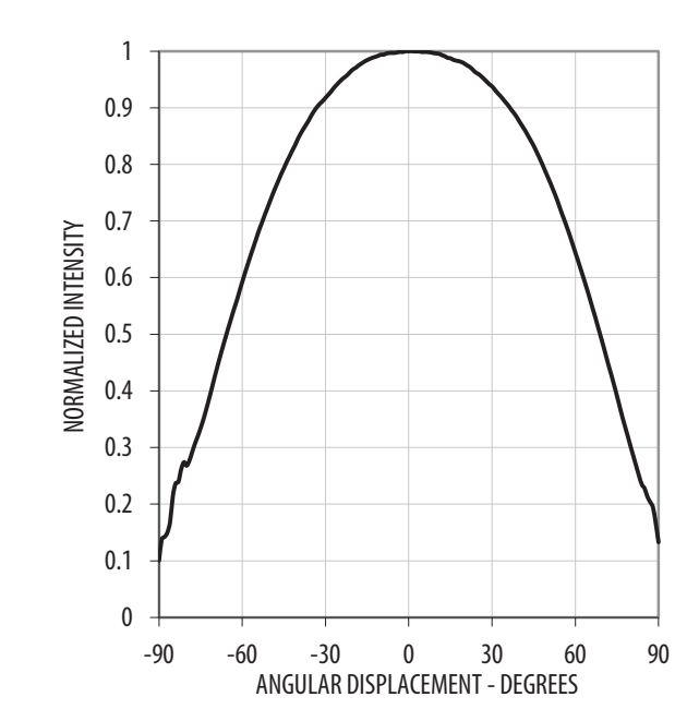
Figure 5: Radiation Pattern
