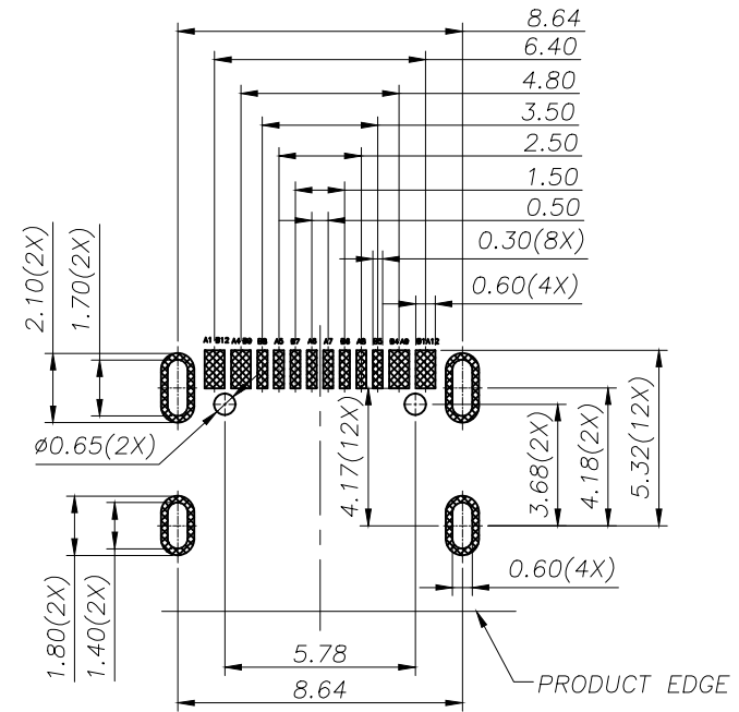
RECOMMENDED PCB LAYOUT(TOP VIEW) THICKNESS 1.60 MM;DEFAULT TOLERANCE:±0.05
