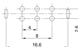
RECOMMENDED PCB LAYOUT TOLERANCE:±0.05
