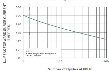
Fig.6 Maximum Non-Repetitive Peak Forward Surge Current
