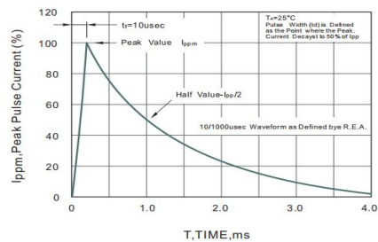
Fig.3 Pulse Waveform
