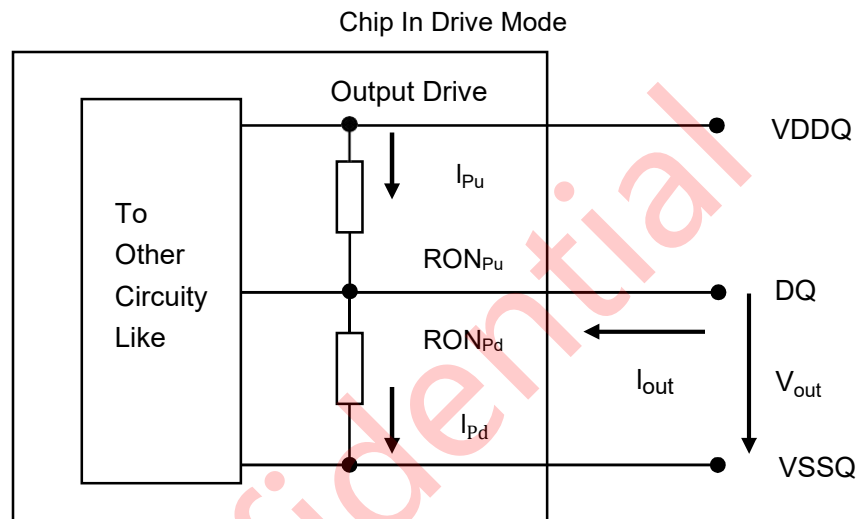
Figure 15 – Output driver
