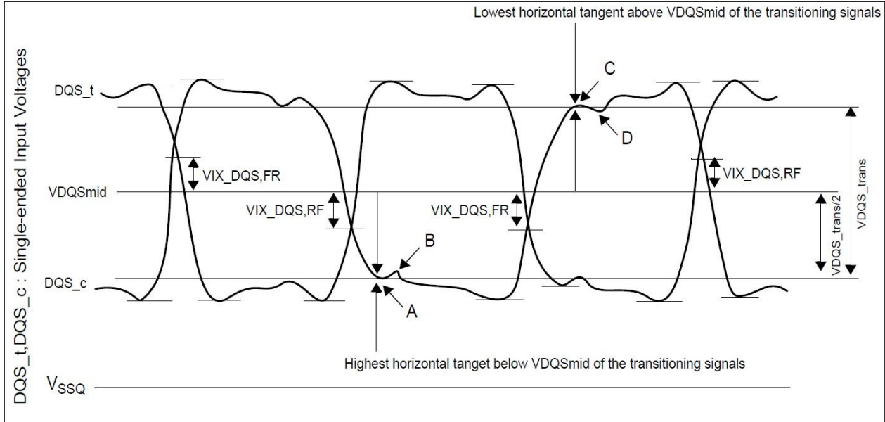
Figure 13 —Vix Definition (DQS)
