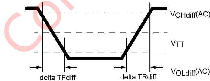
Figure 17 – Differential Output Slew Rate Definition
