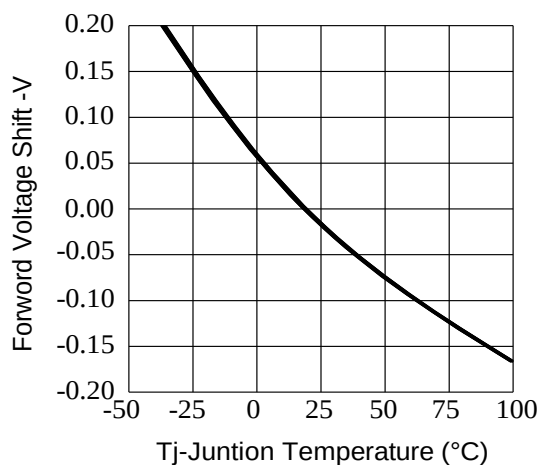
Fig.1-Forward Voltage Shift vs. Junction Temperature
