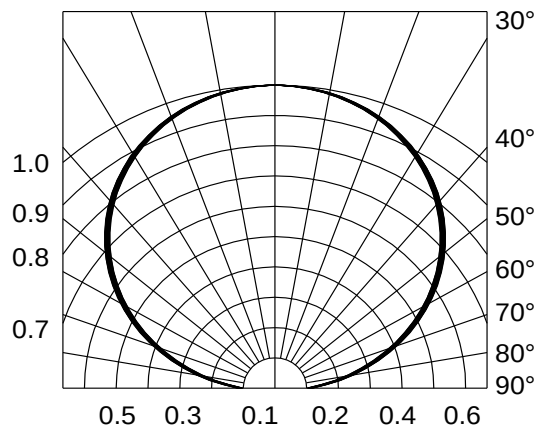
Fig.6-Radiation Diagram
