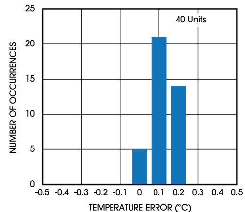
Figure 20. Temperature Sensor Error Histogram 80^\circ\text{C}
