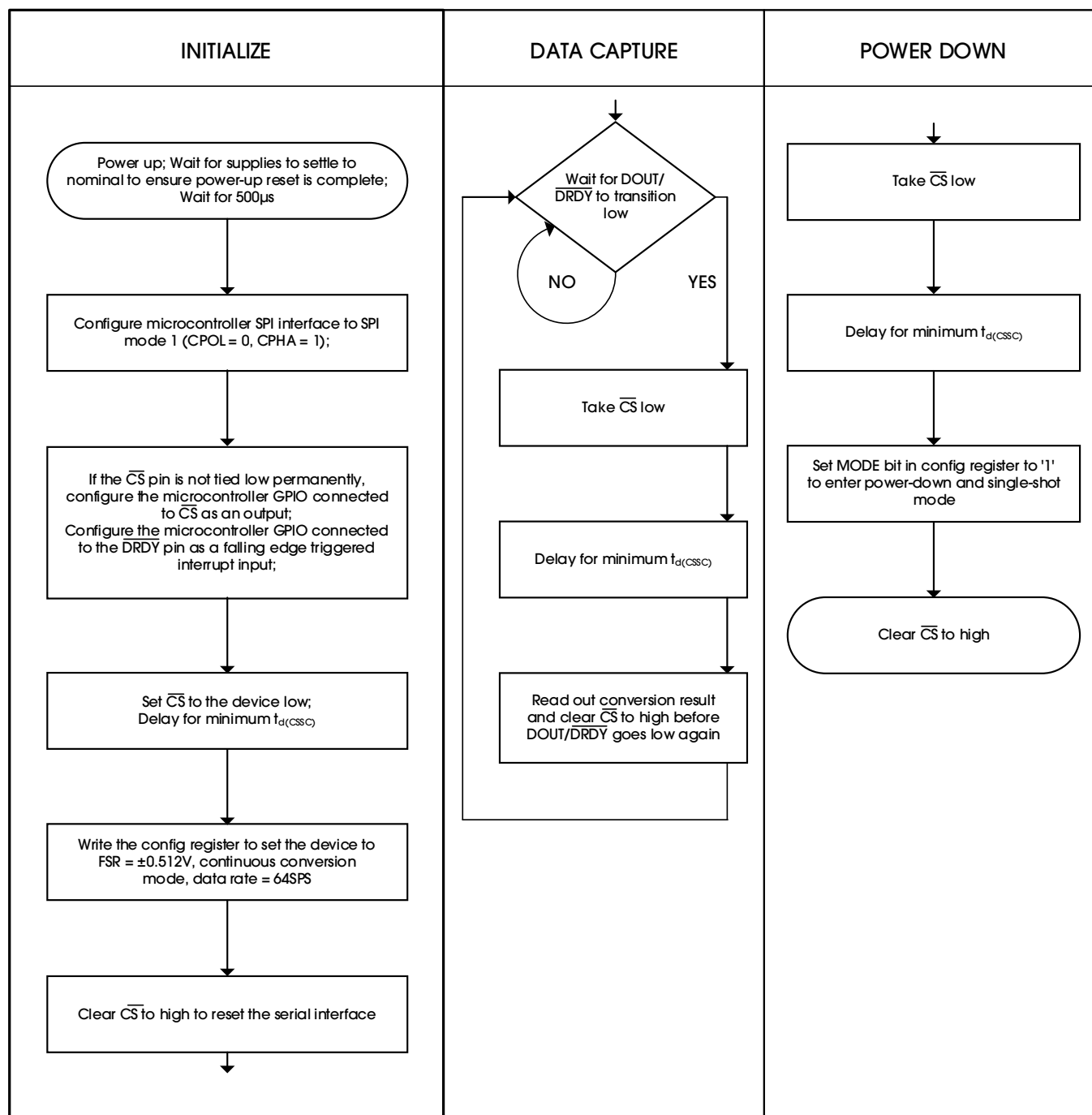
Figure 35. Pseudo Code Example Flow Chart
