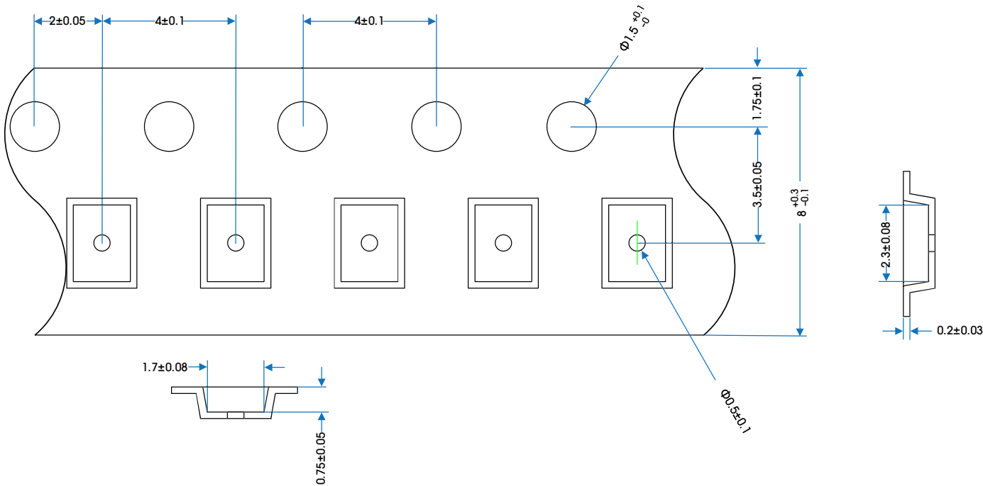
Figure 43 illustrates the carrier tape (QFN-10 package).
