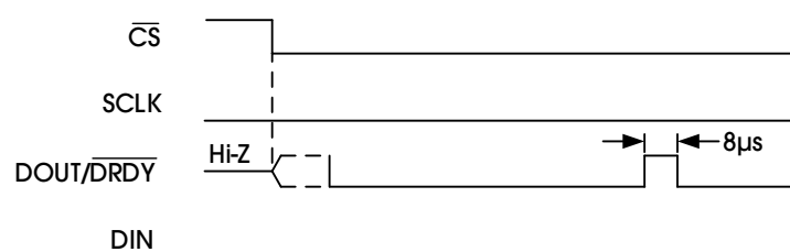
Figure 26. DOUT/ \overline{\text{DRDY}} Behavior without Data Retrieval in Continuous Conversion Mode
