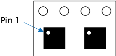
Figure 44. Product Loading Orientation (QFN-10 Package)
