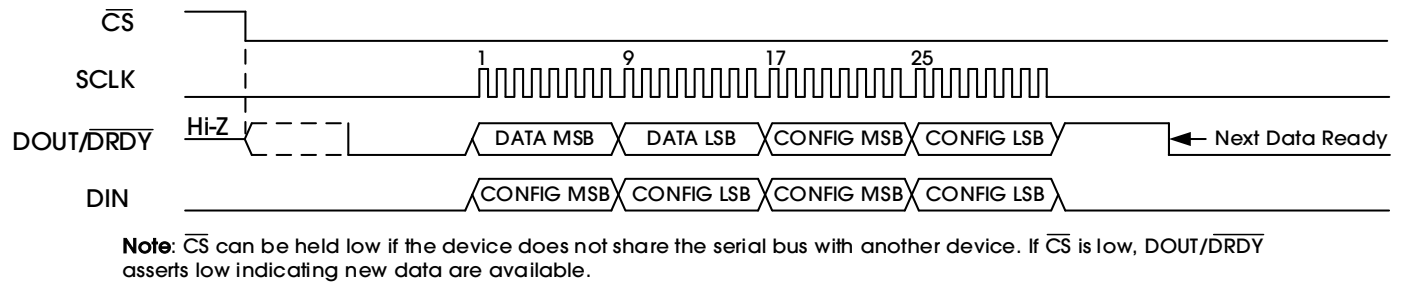
Figure 28. 32-Bit Data Transmission Cycle with Config Register Readback
