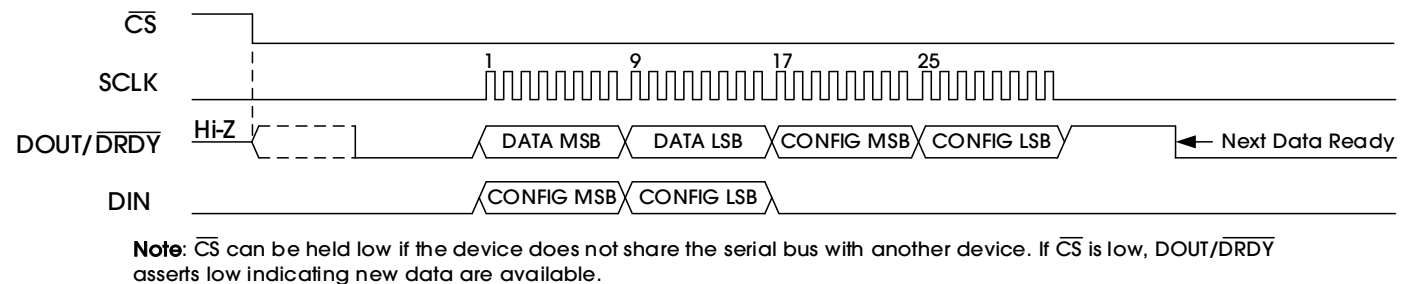
Figure 29. 32-Bit Data Transmission Cycle: DIN Held Low
