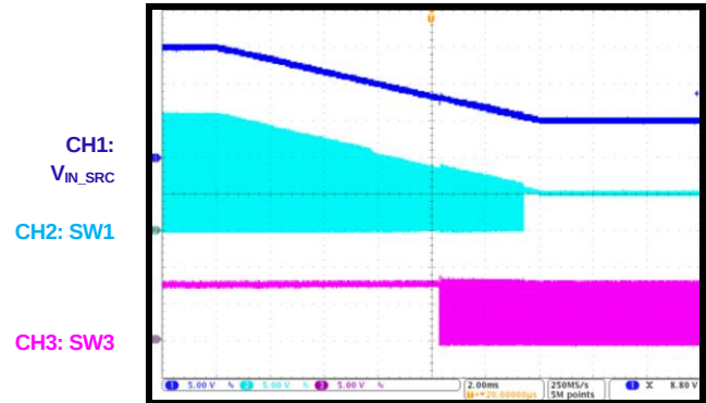
V IN_SRC Step from 15V to 5V
