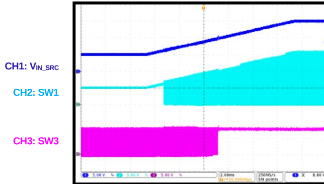
V IN_SRC Step from 5V to 15V
