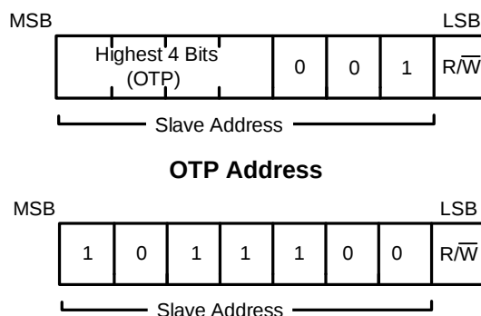
Figure 14: 7-Bit Address
