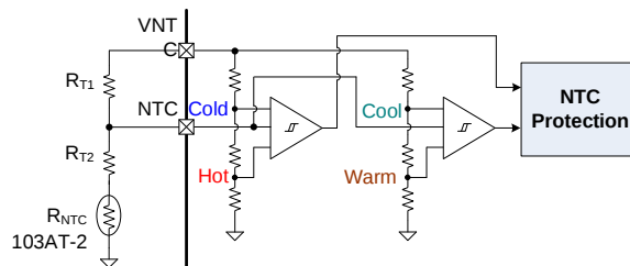
Figure 10: NTC Protection Circuit
