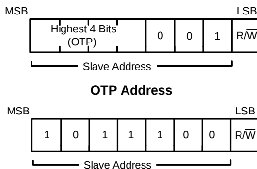
Figure 14: 7-Bit Address
