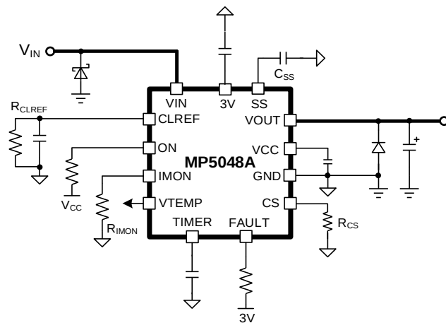
Figure 7: Standalone Operation
