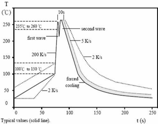
Typical values (solid line). Process limits (dotted line). 波峰焊 (WAVE Soldering)
