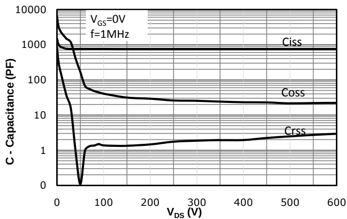
Fig 11: Capacitance Characteristics
