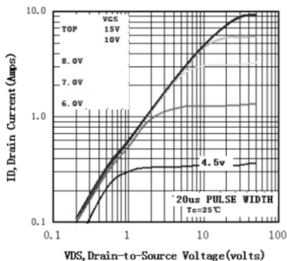
Figure 1. Typical Output Characteristics T_c=25^\circ\text{C}
