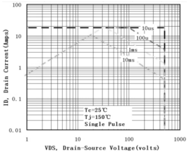
Figure 6-2. Maximum Safe Operating Area TO-220
