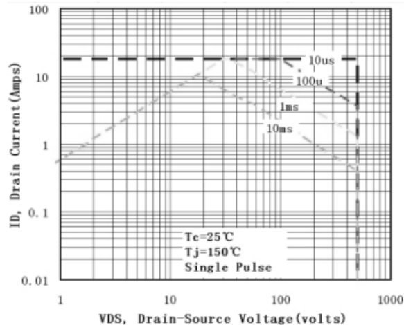
Figure 6-1. Maximum Safe Operating Area TO-220F
