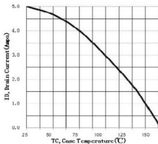
Figure 5. Maximum Current VS Case Temperature
