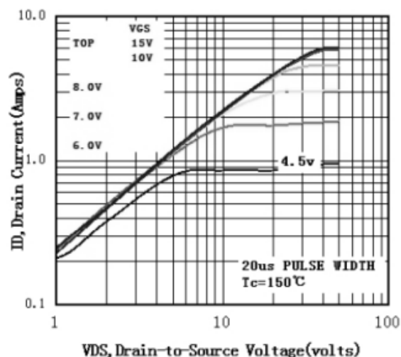
Figure 2. Typical Output Characteristics T_c=150^\circ\text{C}
