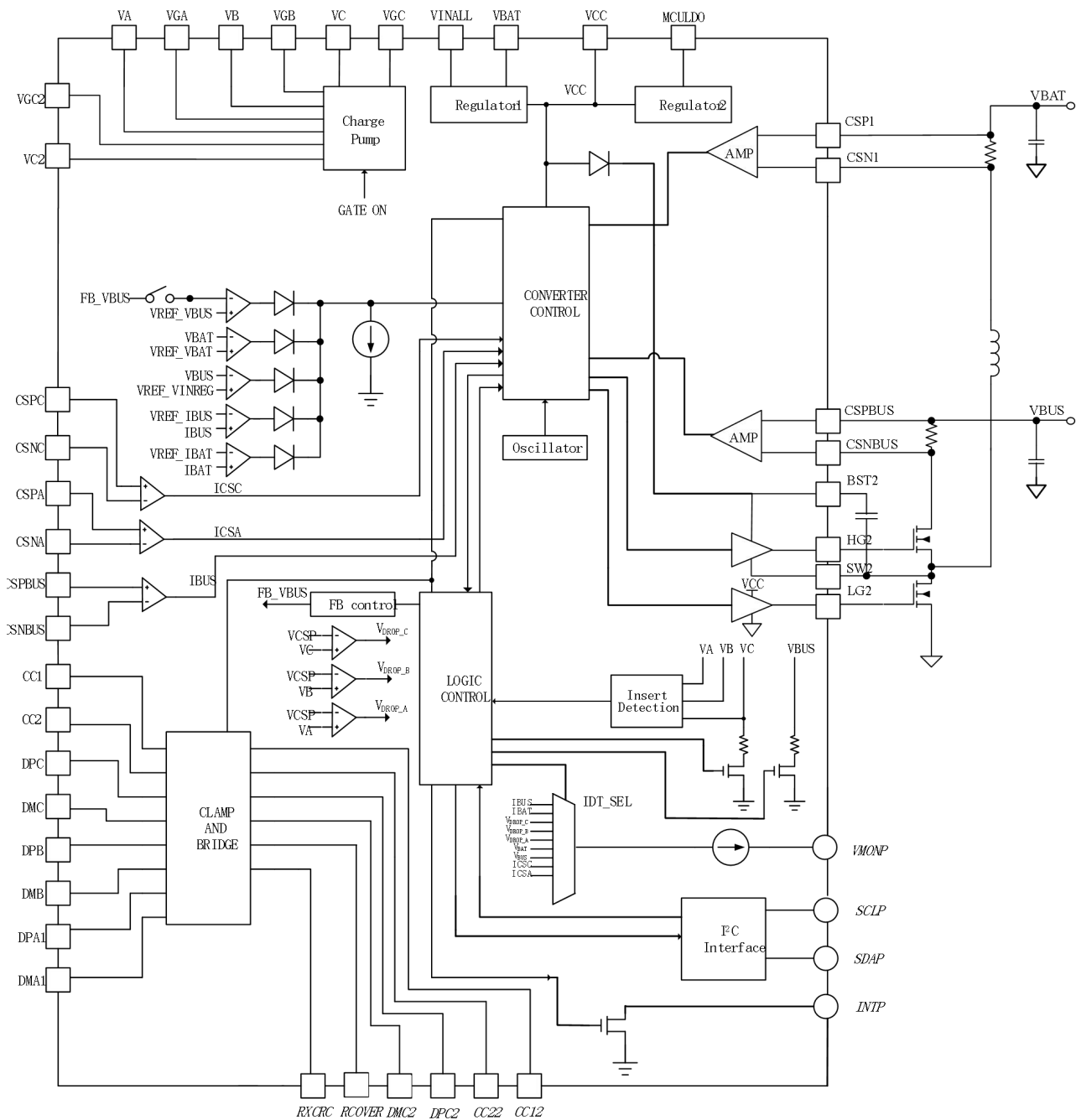
Fig. 8-2-1 PL62005 Diagram
