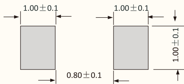
Recommended Pad Layout (mm) 建议焊盘布局(mm)
