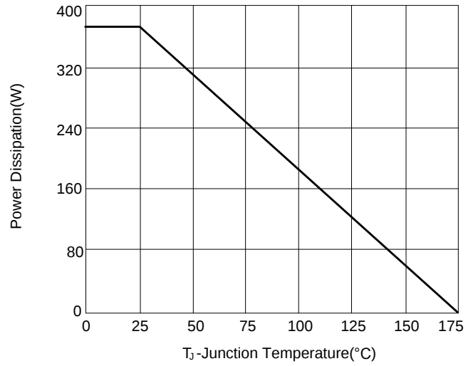
Figure 8: Power De-rating
