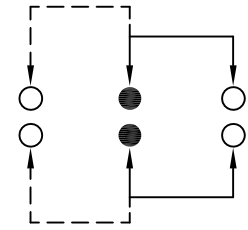
SCHEMATIC (NON-SHORTING)
