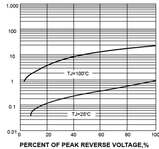
FIG. 4-TYPICAL REVERSE CHARACTERISTICS
