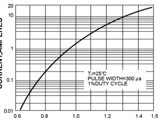
FIG. 3-TYPICAL INSTANTANEOUS FORWARD CHARACTERISTICS
