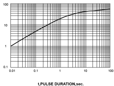
FIG. 6-TYPICAL TRANSIENT THERMAL IMPEDANCE
