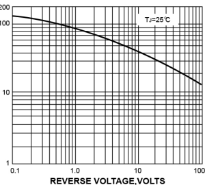
FIG. 5-TYPICAL JUNCTION CAPACITANCE
