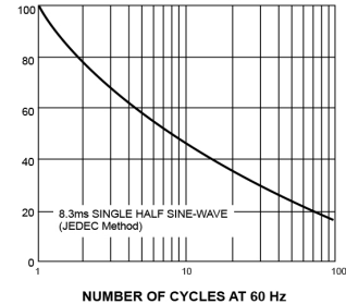
FIG. 2-MAXIMUM NON-REPETITIVE PEAK FORWARD SURGE CURRENT
