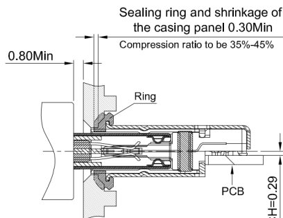
RECOMMENDED ASSEMBLY TOLERANCE:±0.03mm
