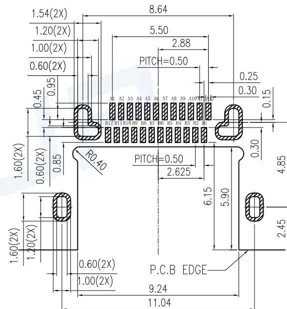
RECOMMENDED PCB LAYOUT(TOP VIEW) THICKNESS 0.60MM;DEFAULT TOLERANCE:±0.05
