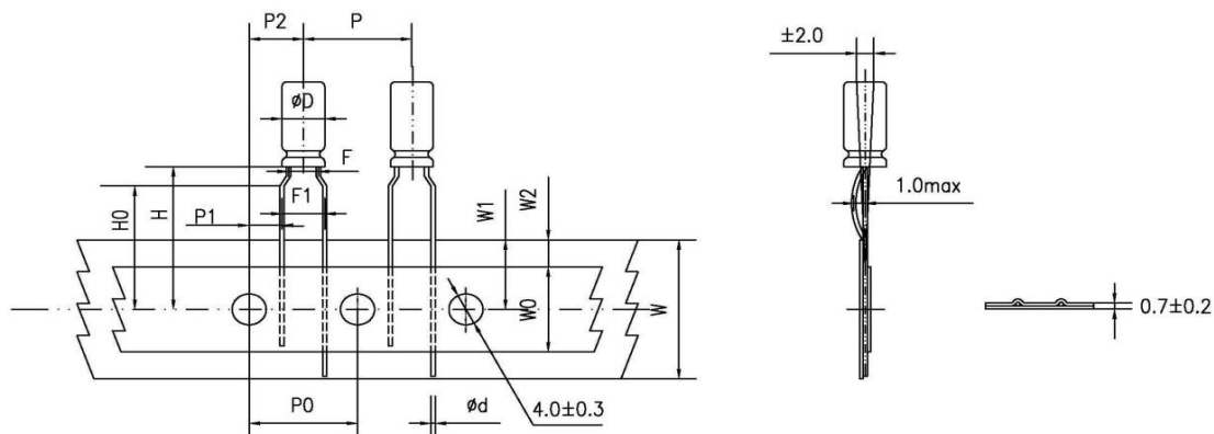
DIMENSIONS(mm)
