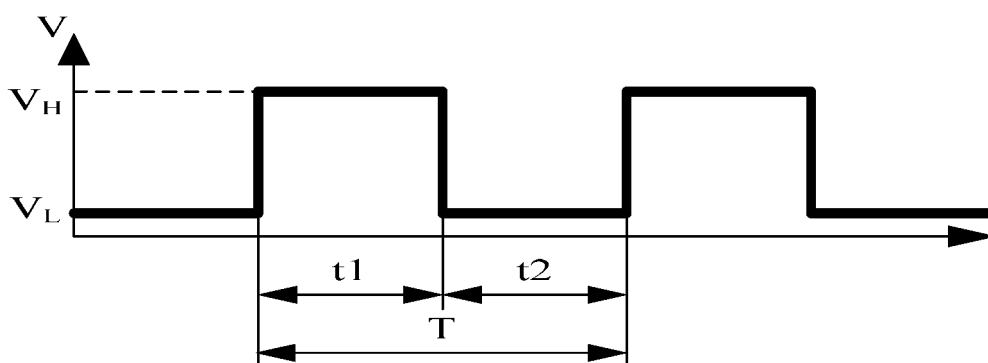
★PWM INPUT WAVEFORM
