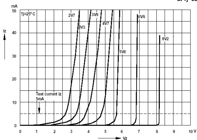
Breakdown characteristics at T_J=\text{constant} (pulsed)
