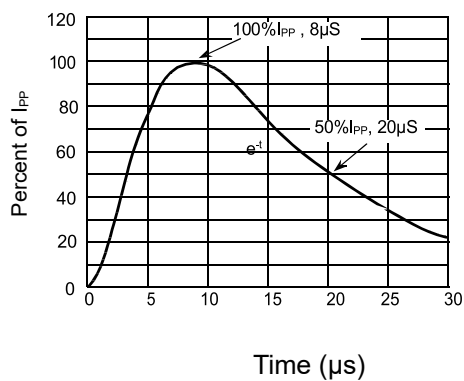
Figure 3: Pulse Waveform-8/20 \mu s
