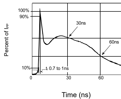
Figure 4: Pulse Waveform-ESD(IEC61000-4-2)
