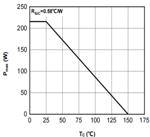
Fig.11 Max. power dissipation vs case temperature
