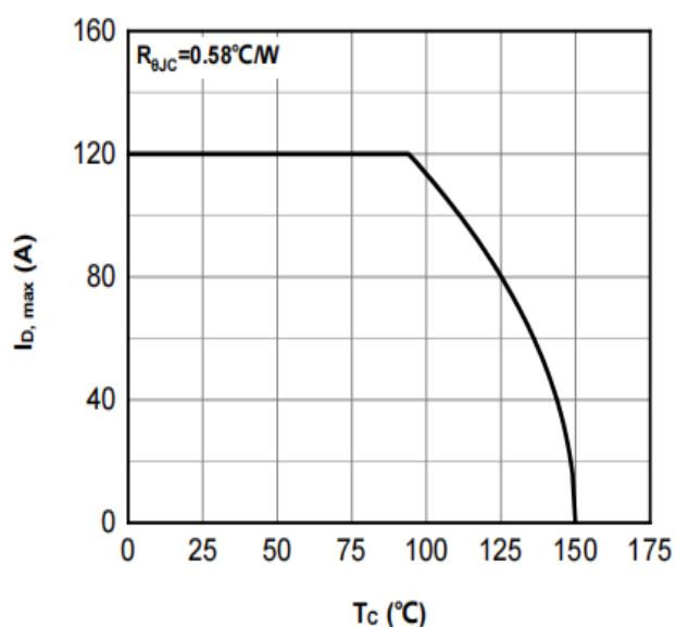
Fig.12 Max. continuous drain current vs case temperature
