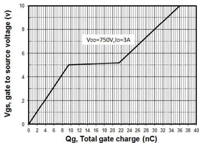
Figure 14. Typical Gate Charge
