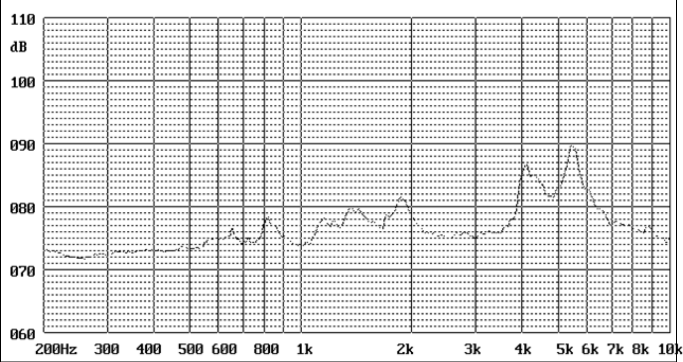
Typical Frequency Response Curve (音频曲线图)
