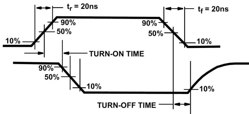
Figure 2. Waveforms, Channel Being Turned ON( R_L = 1\text{ k}\Omega )
