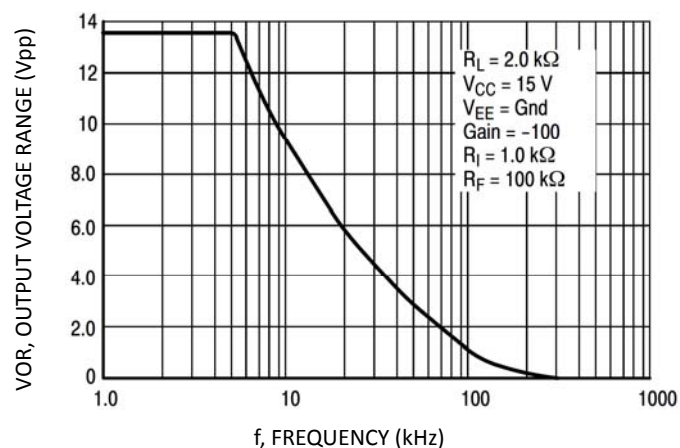
Large-Signal Frequency Response
