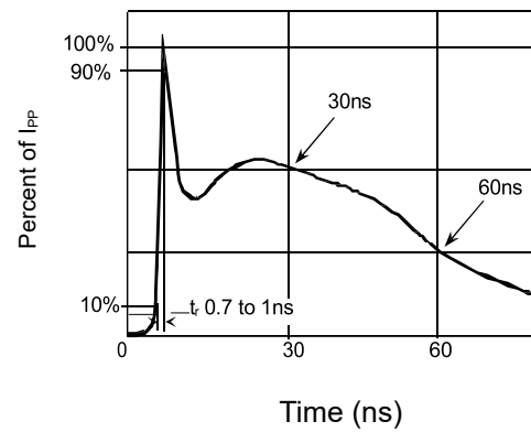
Figure 4: Pulse Waveform-ESD(IEC61000-4-2)
