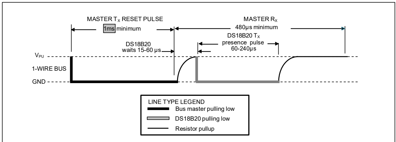
Figure 13. Initialization Timing
