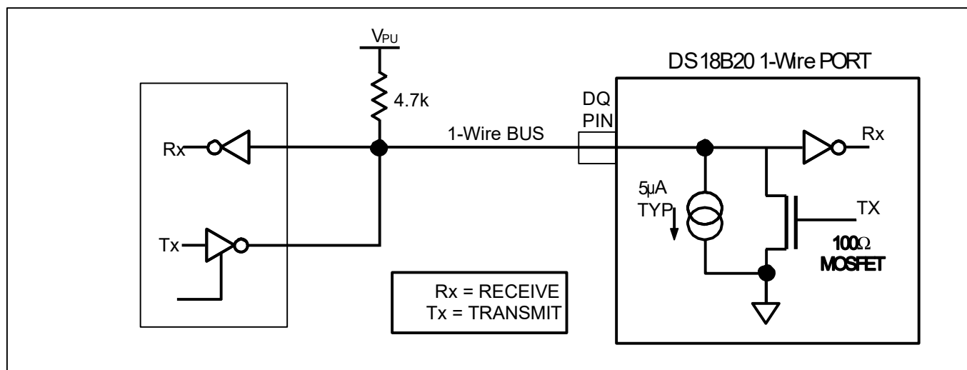
Figure 10. Hardware Configuration
