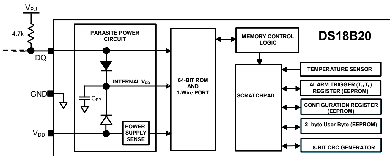
Figure 1. DS18B20 Block Diagram
