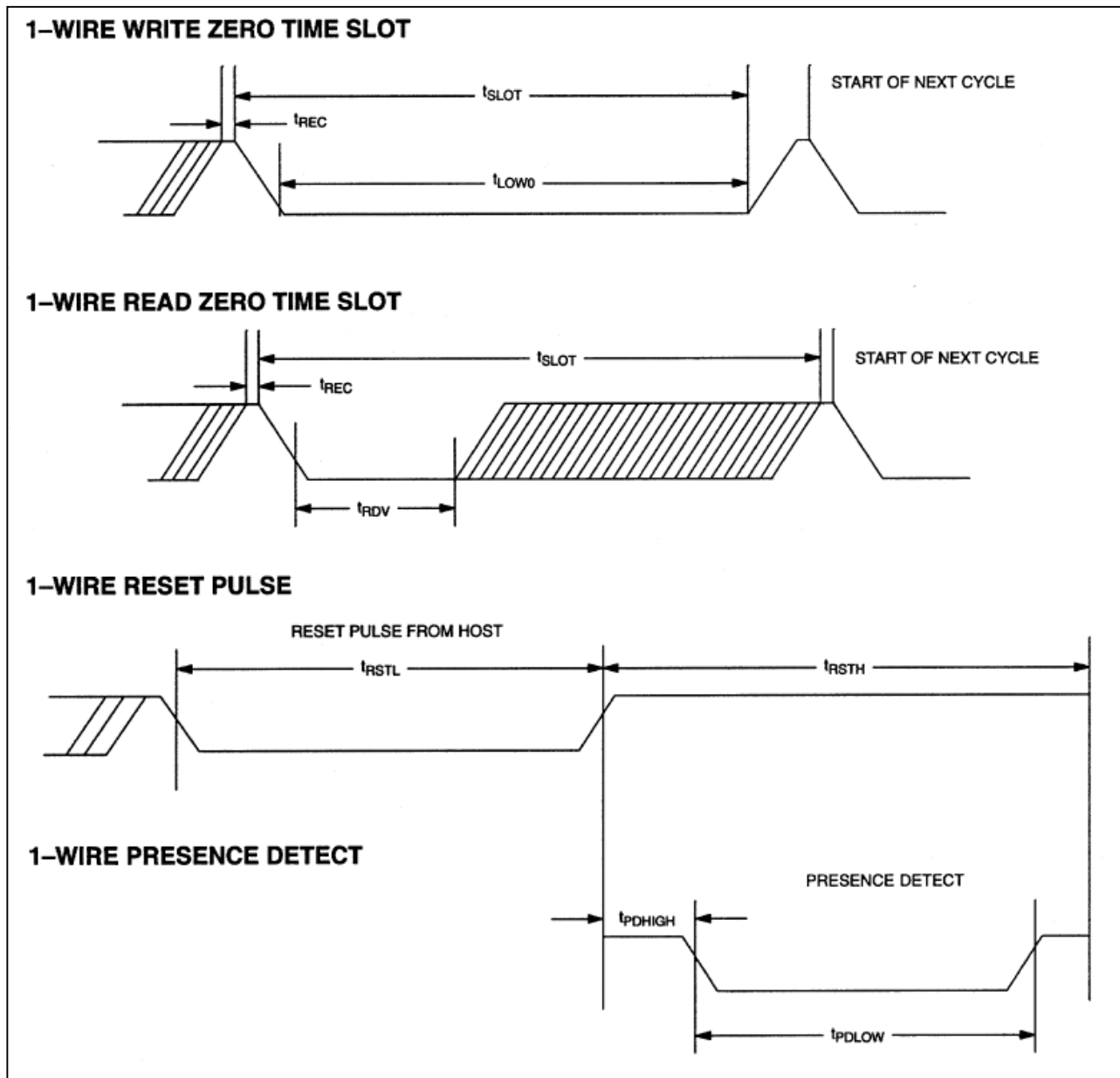
Figure 18. Timing Diagrams
