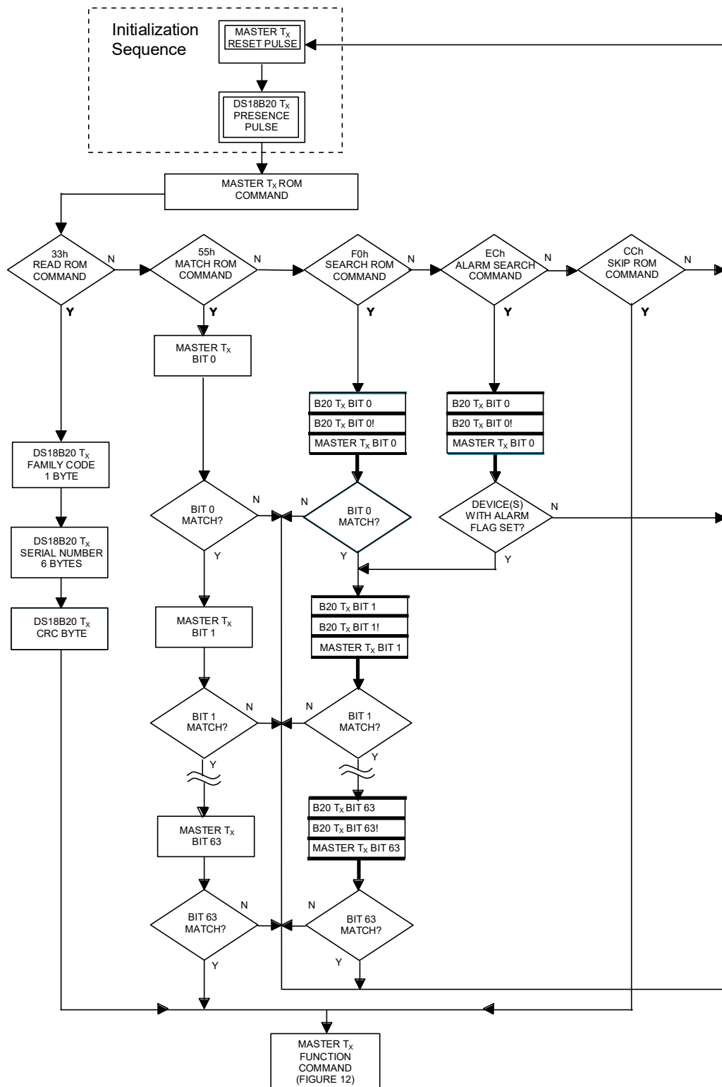
Figure 11. ROM Commands Flowchart
