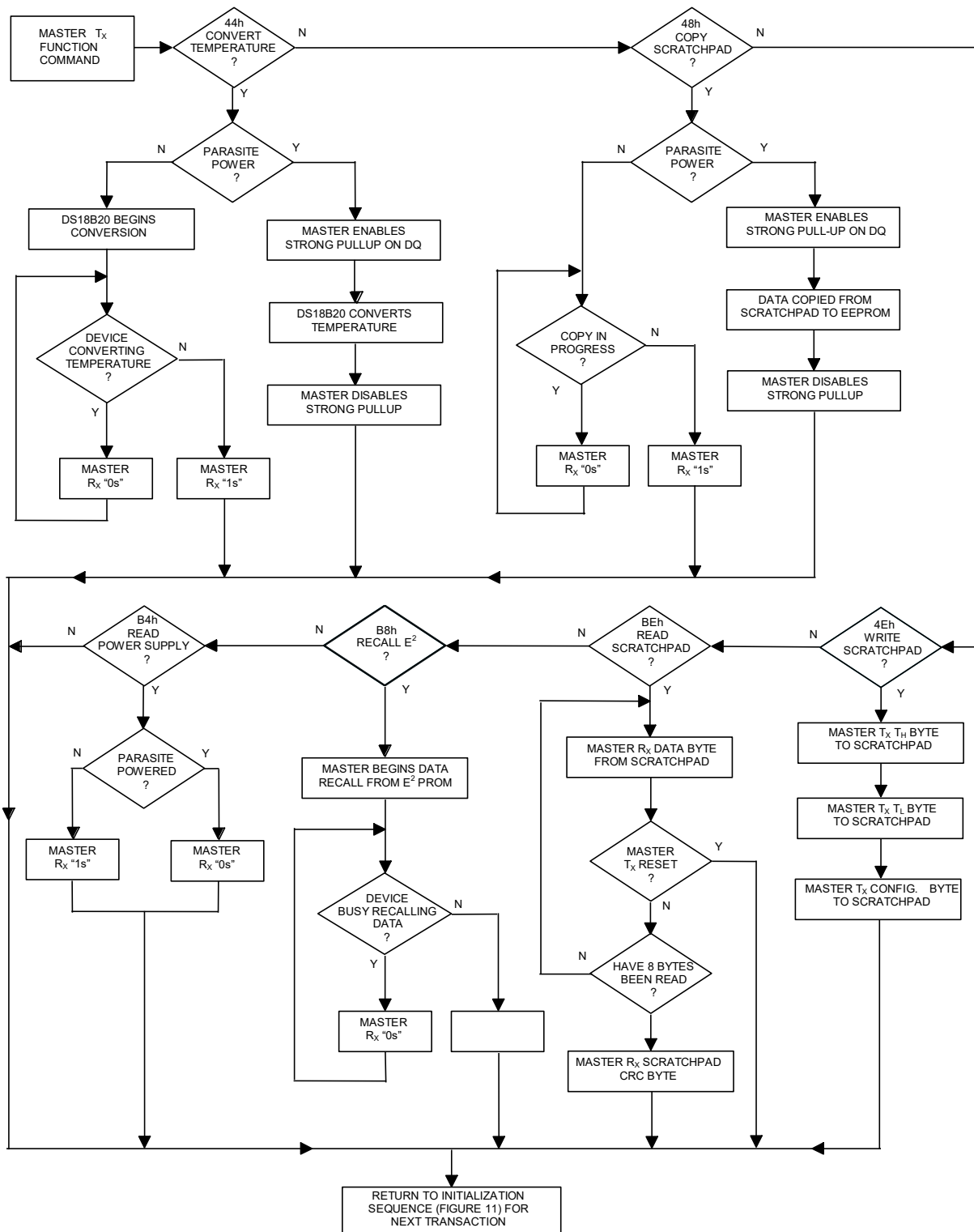
Figure 12. DS18B20 Function Commands Flowchart
