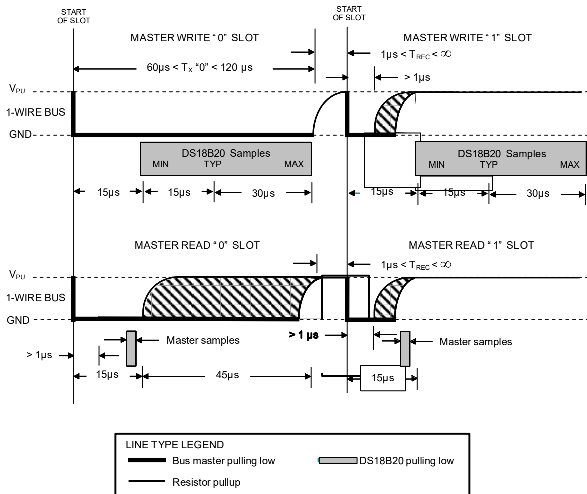
Figure 14. Read/Write Time Slot Timing Diagram
