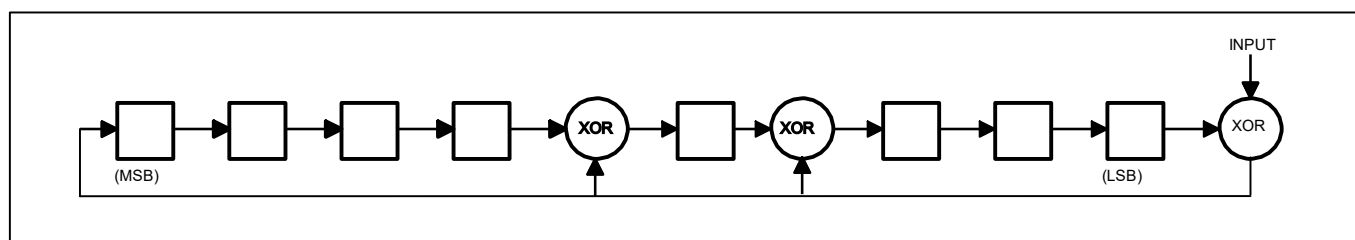
Figure 9. CRC Generator
