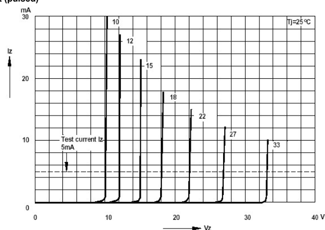
Breakdown characteristics at Tj=constant (pulsed)
